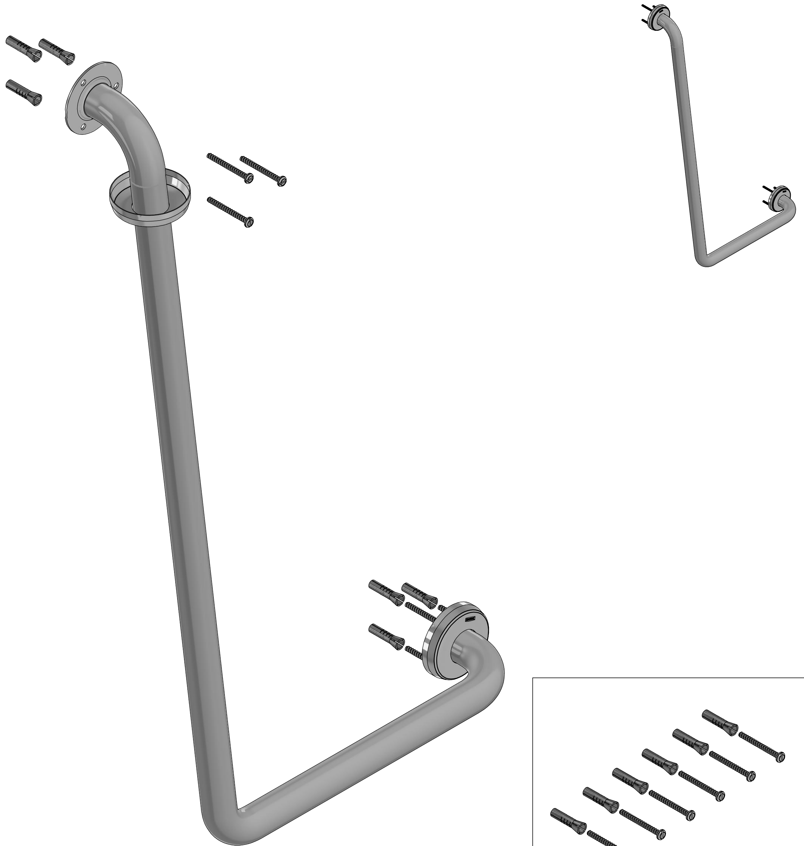
Sa-125 Taquetes de Plomo-3 y Pija 10-16 x 2" Plugs Lead-3 and Lag Screw 10-16 x 2"
